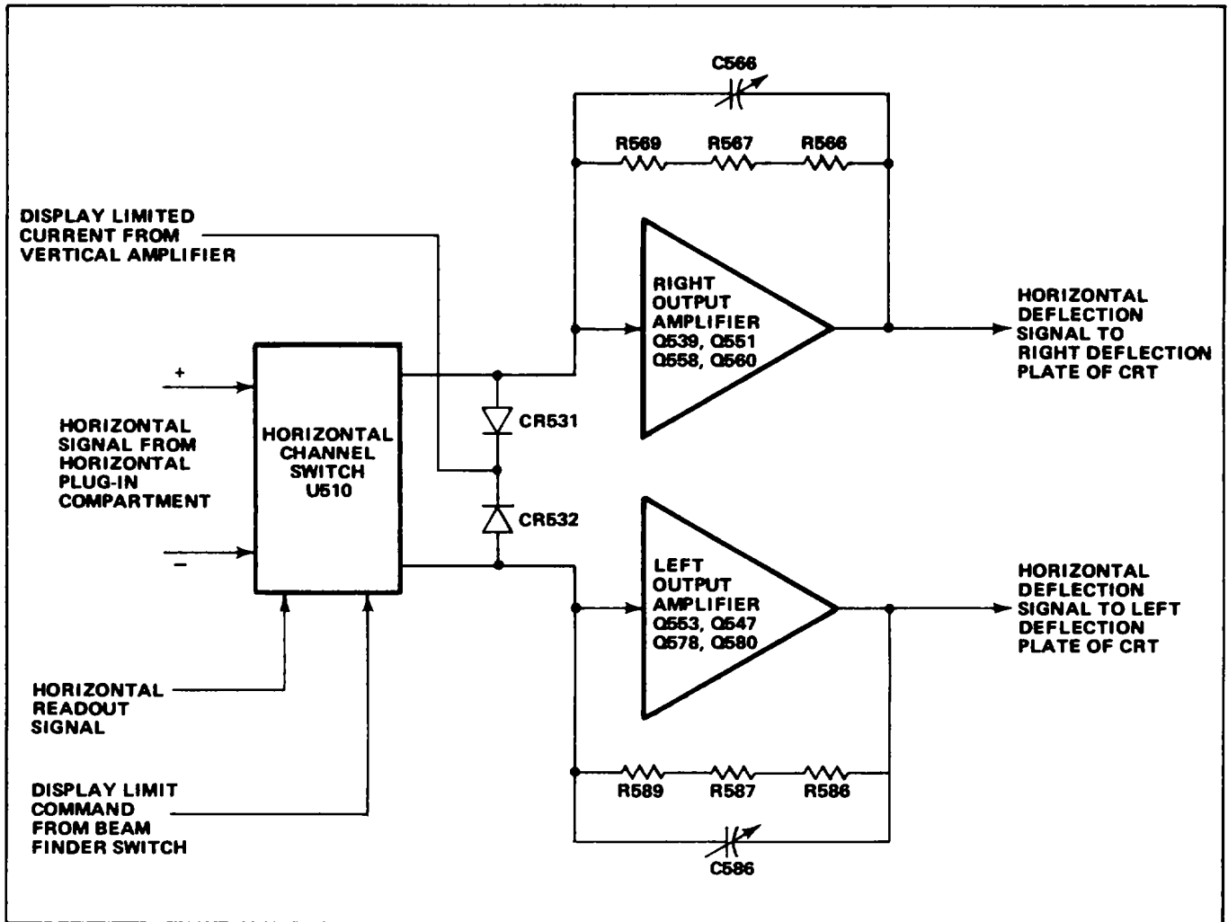
Figure 3-19. Horizontal Amplifier
