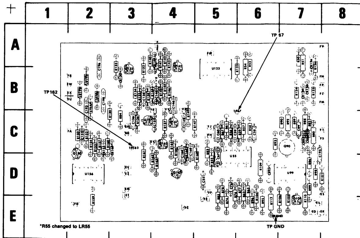
Figure 8-3. A2-Logic board.
