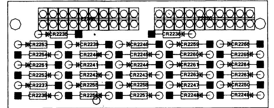
Figure 8-15A. A18-Protection circuit board (SN B14000-up).
