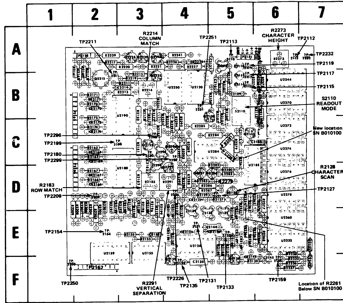
Figure 8-15. A13-Readout board.
