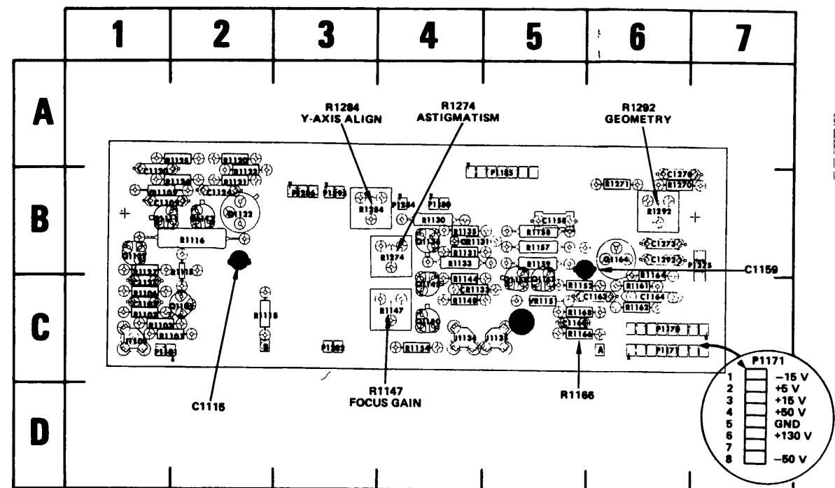
Figure 8-10. A8-Z-Axis board.
