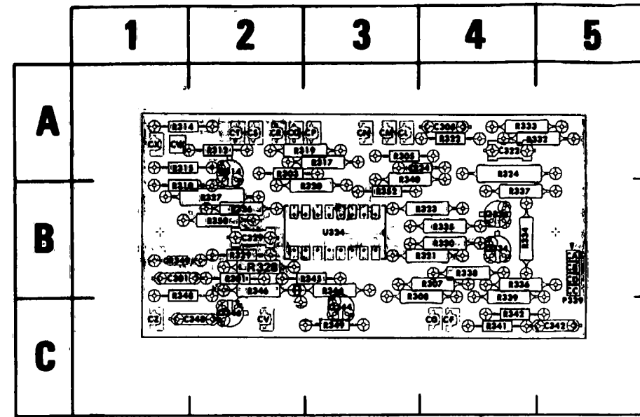
Figure 8-4. A3-Trigger Selector board.
