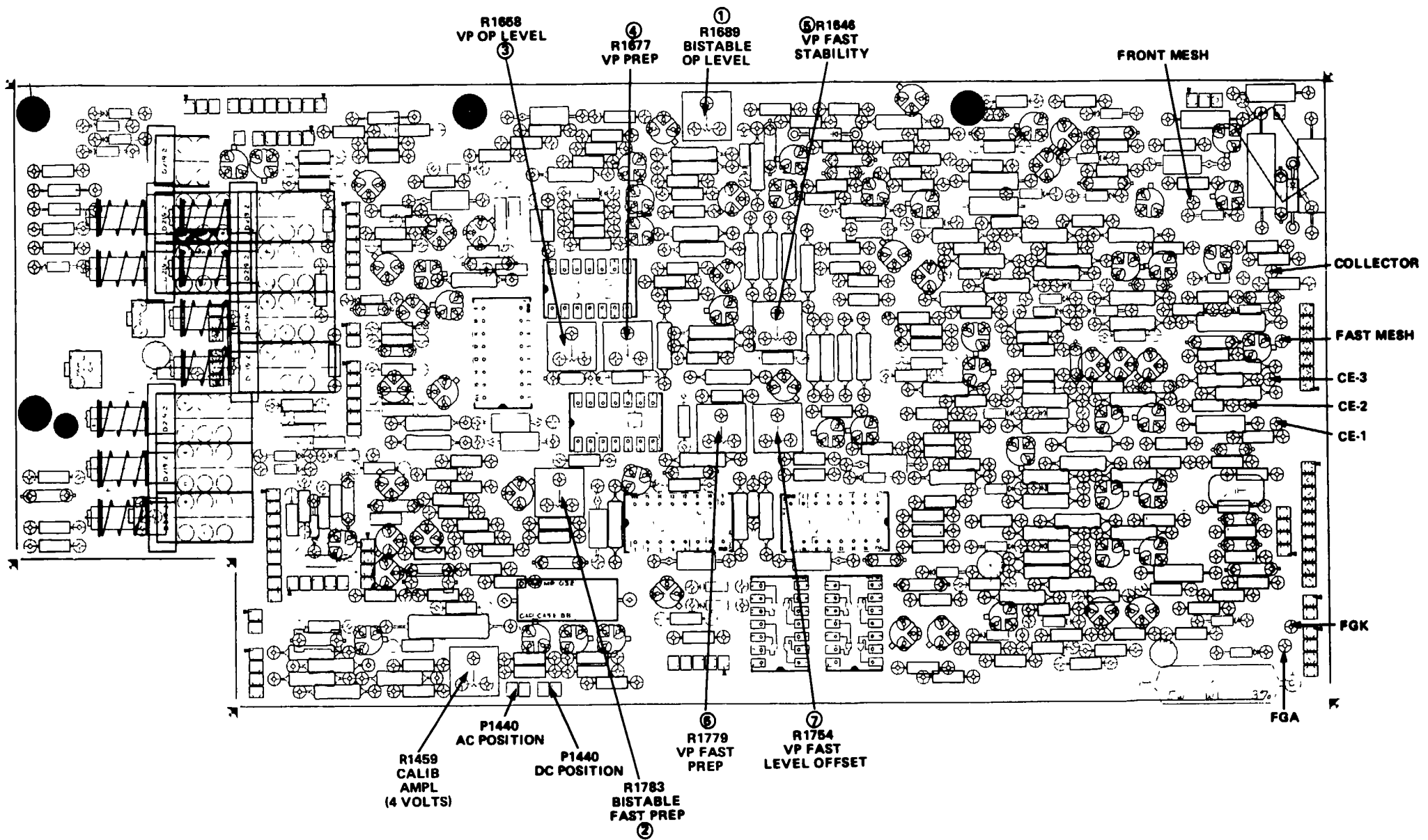
Figure 8-24. Storage board.
