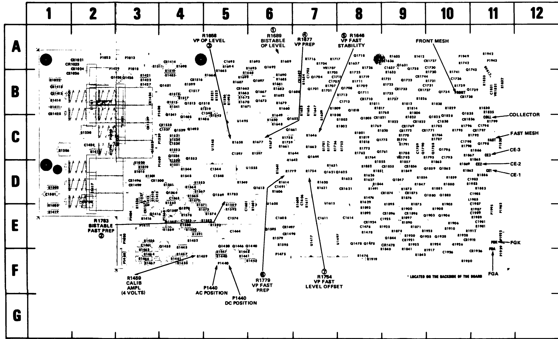
Figure 8-16B. A14-Storage board, SN B129999-below.
